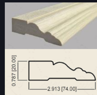
OTG029- Casing
