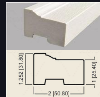
OTG006- Notched Back Brickmould
